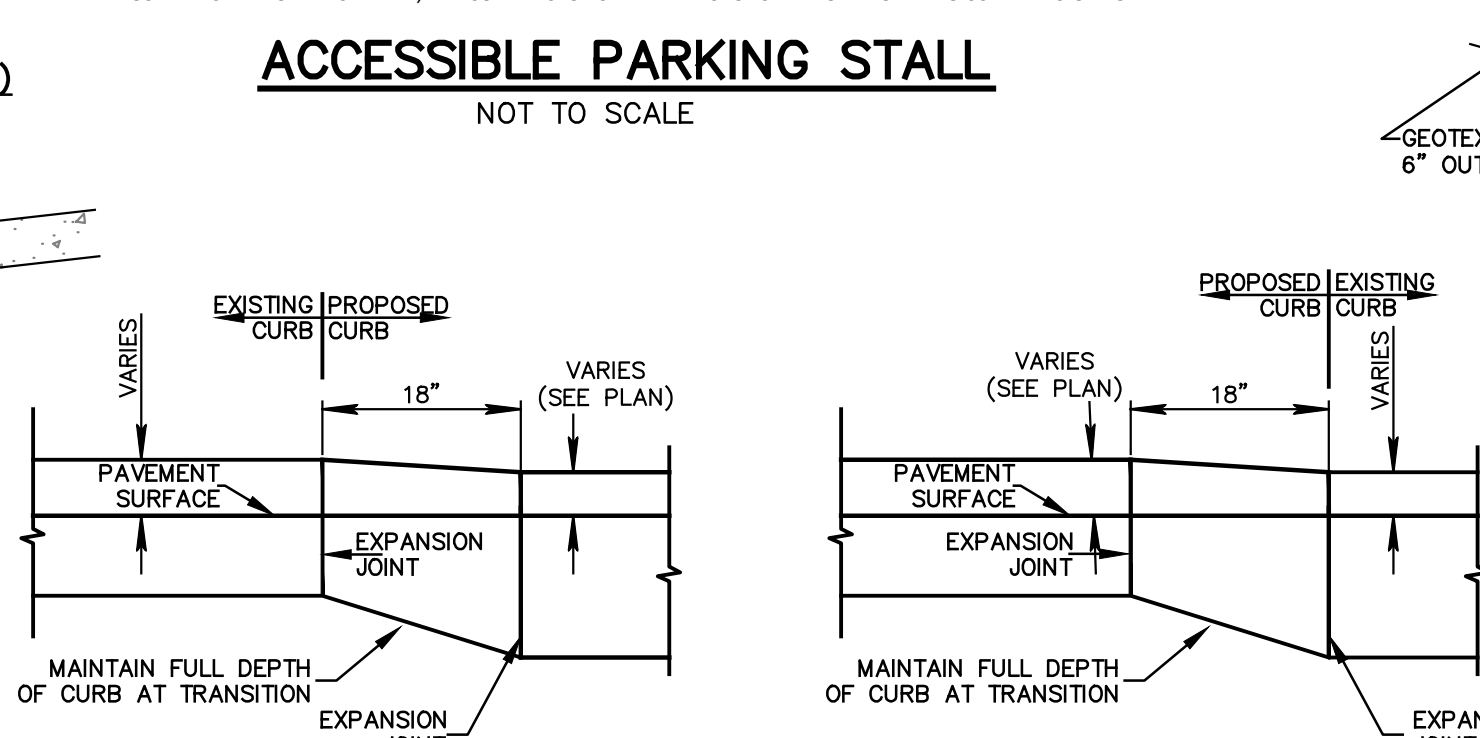
TRANSITION TO EXISTING CURB
