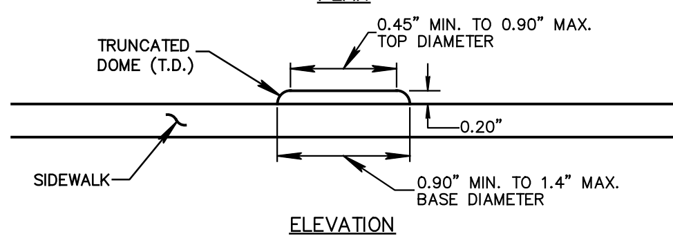
DETECTABLE WARNING SURFACE
