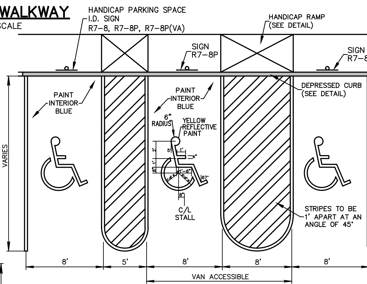
ACCESSIBLE PARKING STALL
