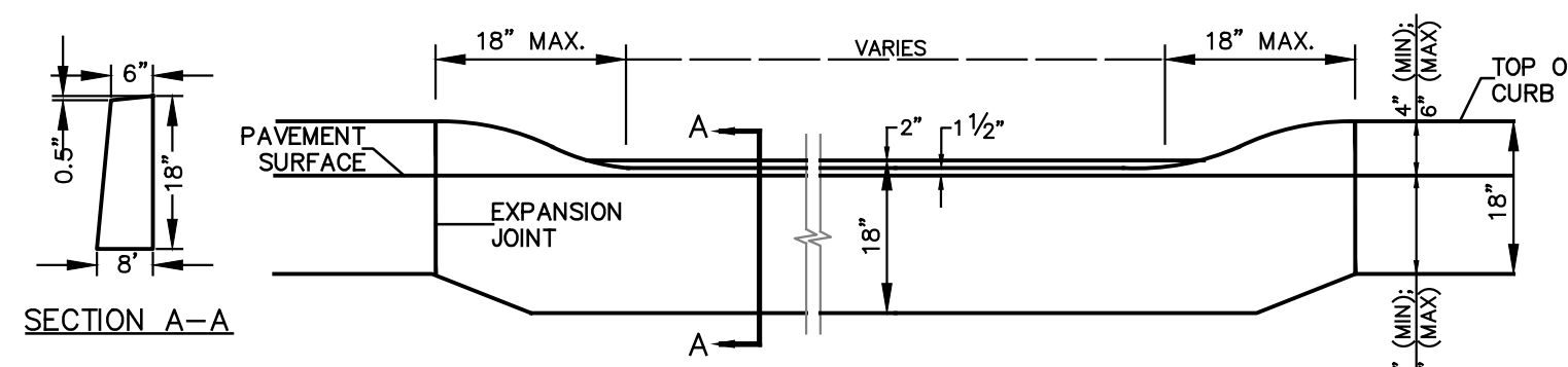
DEPRESSED CURB
