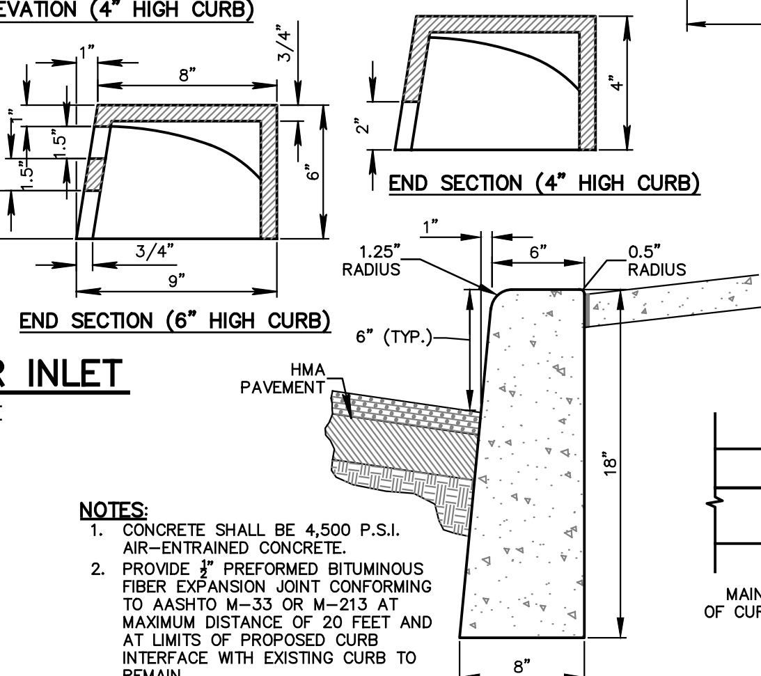
CONCRETE CURB
