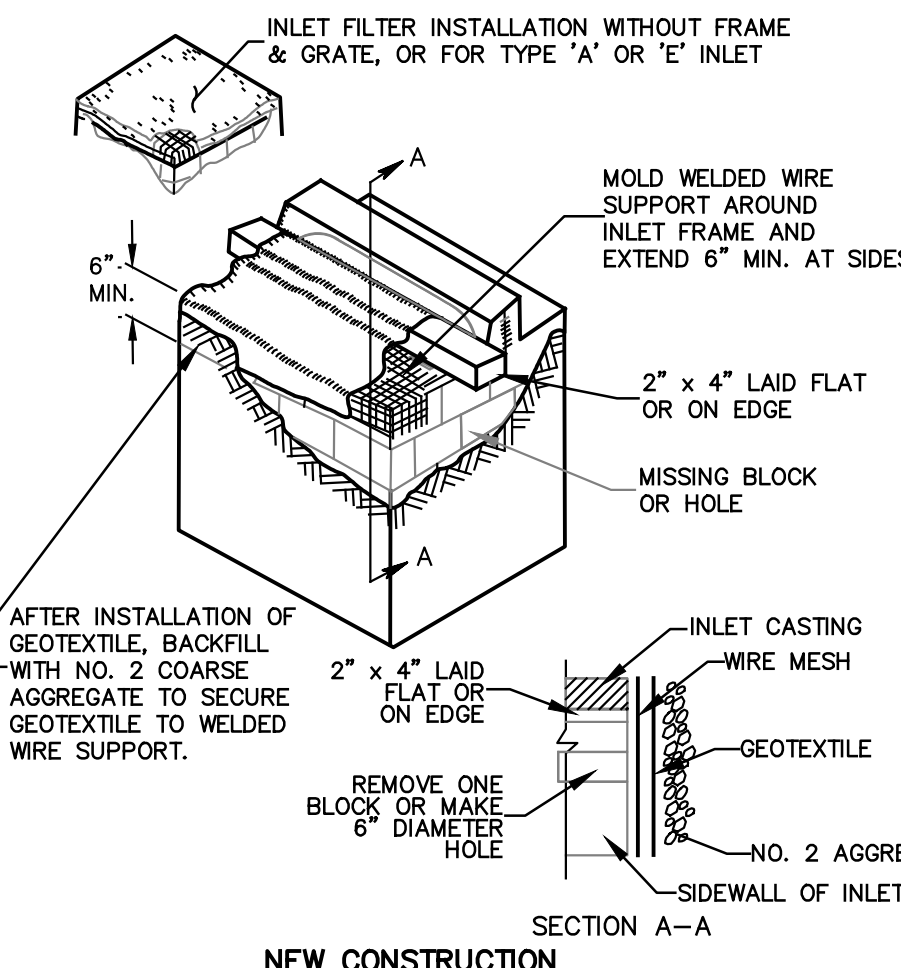
INLET PROTECTION
