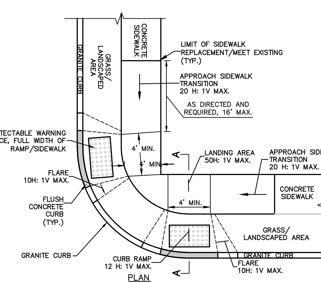
TYPICAL ACCESSIBLE RAMPS
